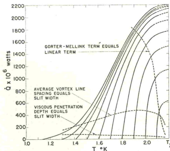
FIG. 4. Family of heat flow curves as calculated using Eq. (26); d = 3.36 \mu , v_c = 0 , A as given by Vinen (4). Dashed lines across the heat flow curves indicate several regions useful in interpreting the vortex line model used for the calculations (see Section V).
